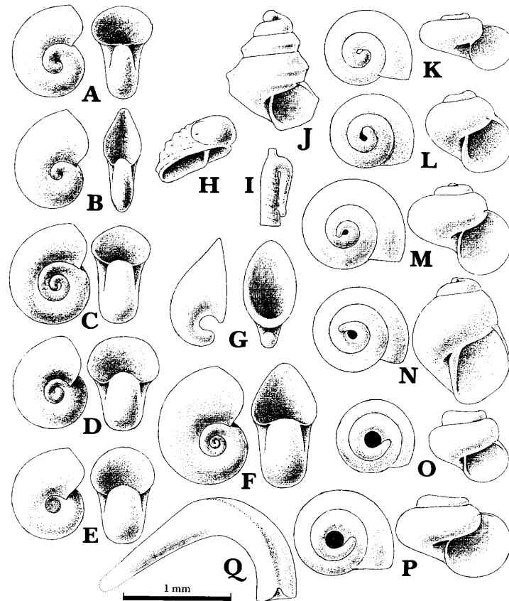
Fig. 23. Diversity of larval and early postlarval gastropod and bellerophonitid conchs in sample 129s taken at depth 1337 of the Lesieniec borehole, eastern Poland; early Caradoc, Baltioniodus variabilis Subzone. Semidiagrammatic presentation based on camera lucida drawings of phosphatized conchs; growth lines are rarely discernible in the Lesieniec material. □A. Severynella trochlearis Hynda 1983 (3.9 per cent of the assemblage). □B. Temnodiscus disciformis Hynda 1983 (3.2). □C. cf. Bucania christianaie (Koken 1925) (2.6). □D. Kokenospira? sp. aff. K. subglobosa Hynda 1983 (3.8). □E. Sinuities sp. (0.1). □F. Tropidodiscus ( Peruniscus ) minimus Hynda 1983 (29.8). □G. Archinacella? sp. (0.9). □H. Mimospira sp. (6.6). □I. Jinonicella sp. n. (0.8). □J. Trochonema sp. (2.6). □K. ' Straparollus ' sp. (2.9). □L. Holopea? sp. aff. H. pusilla Hynda 1986 (29.4). □M. ' Naticonema ' sp. (2.7). □N. Subulites cf. revalensis Koken 1925 (0.8). □O. Subulitid similar to PMO NF 3207/5, 4 in Bockelle & Yochelson (1979: Fig. 5F–H) (2.5). □P. Clathrospira? obscura (Hynda 1986) (3.1). □Q. Eccyliomphalus , Leseurilla or Pararaphistoma sp. (4.3).
