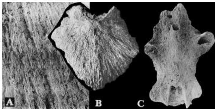
Fig. 19. Phosphatized meroms of the Ordovician receptaculite Tetragnis munchisoni Eichwald 1840 showing originally aragonitic radial acicular structure; borehole Lesieniec 1, eastern Poland, sample S-129s, early Caradoc. □A–B. Corroded head plate from inner side, \times 225 and 45 , respectively. □C. Head from internal side with partially preserved bases of horizontal spines; \times 60 .
