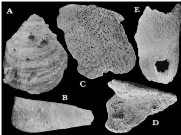
Fig. 21. Phosphatized valves of Ordovician polyplacophorans; all \times 50 except B which is \times 40 . □A. Chelodes sp. late Caradoc of the Mójcza Limestone, Holy Cross Mountains, Poland, sample MA-4, note surface granulation. □B. Solenocaridid Bursata santacrucensis Dzik 1994 from latest Caradoc of the Mójcza Limestone, sample MA-99, lateral view of tail valve. □C-E. Septemchitonid Sarkachiton kielcensis Dzik 1994 from MA-99 (C) and early Caradoc of the Lesieniec 1 borehole, eastern Poland, sample 129s, thoracic (C-D) and tail (E) valves; note spinose appearance of the valve surface.
