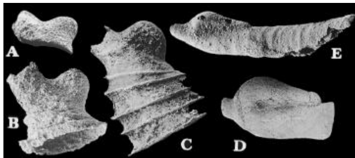
Fig. 13. Early Paleozoic snorkel-bearing minute molluscs: \times 75 . □A–C. Yochelcionella sp. from the bed with opercula at Aččagy Tuoidach, Atdabanian. Ontogenetic series of conchs, now calcitic. □D. Jinonicella sp. n. from early Caradoc sample 129s of Lesieniec 1 borehole, eastern Poland; phosphatized conch with partially exfoliated wall. □E. Jinonicella kolebabei Pokorný 1978 from the Ludlow Kok Formation of Cellonetta Lavinerinne, Carnic Alps, Austria; phosphatic envelope of the conch.
