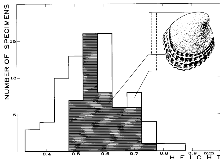
Fig. 33. Size frequency distribution of height of Butovicella valves in randomly selected part of the Cellonetta Lavinerinne sample and height of prodissocoenchs in the whole sample (shadowed). Note that modal values of both histograms are closely similar (although with opposite skewness) which indicates mortality peak exactly at the metamorphosis. At least three species of the cardioids are represented but they do not differ significantly in size of their prodissocoenchs.
