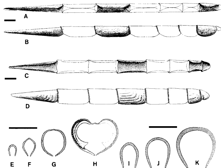
Fig. 29. Reconstruction of body armors of early Palaeozoic solenocaridid Septemchitonida in ventral and lateral views, and camera lucida based cross sections of sclerites of various sizes. Bar scales 500 \mu m. □A–B, E, H. Silurian Carnicoleus gazdzickii Dzik 1986 from the Ludlow of the Carnic Alps, Austria. Specimens E–G from Cellonetta Lavinerinne, H from Rauchkofel Süd. □C–D, I–K. Ordovician Bursata santacrucensis Dzik 1994 from the latest Caradoc of the Holy Cross Mountains, Poland.
