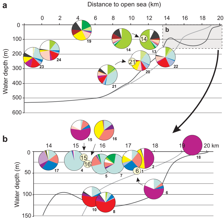
Fig. 6. The 14 most prominent taxa versus water depth and distance to open sea. Gray lines show bathymetrical profiles along the fjord main axes, dark gray for the main channel and Ezcurra Inlet, bright gray for Martel Inlet. For colors assigned to different taxa, see Fig. 5.
