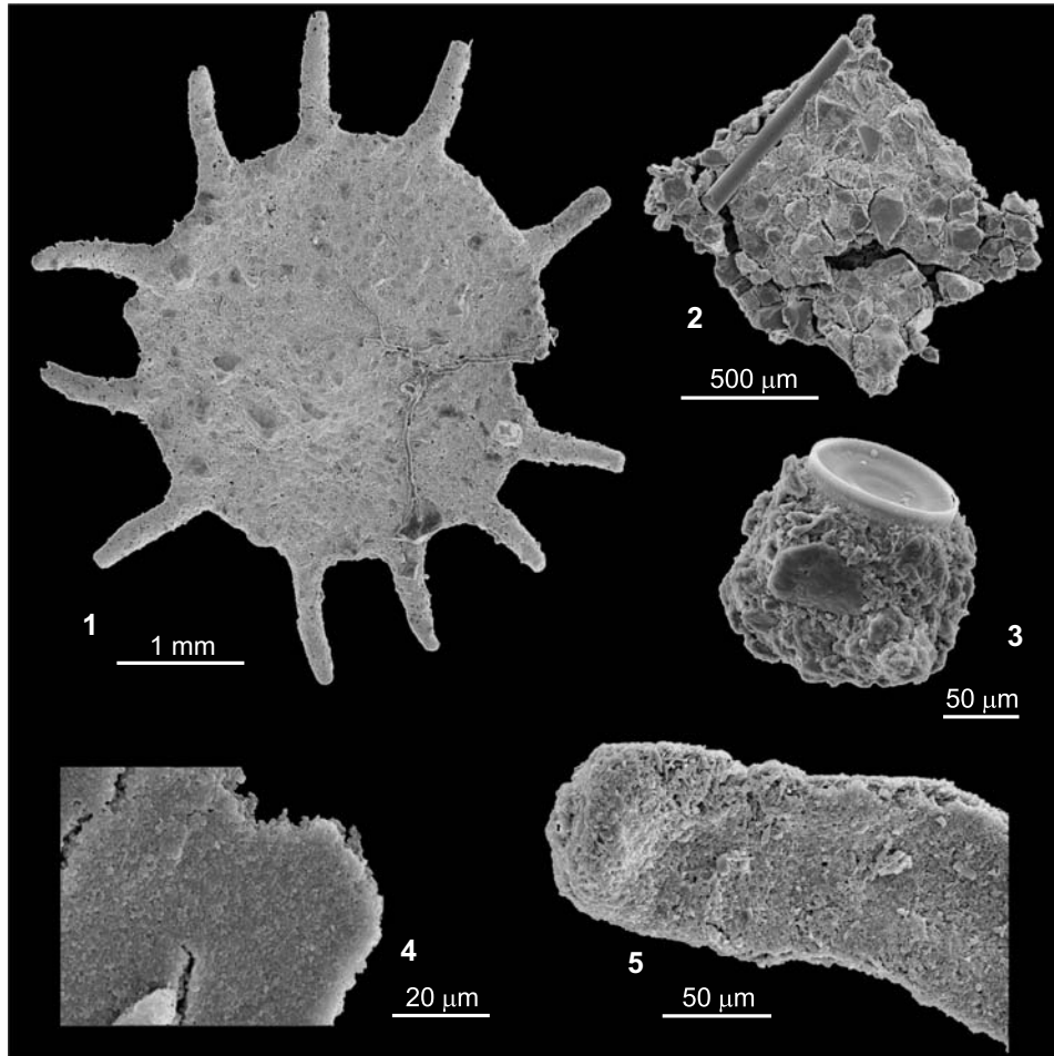
Fig. 7. 1. Astrorhiza sp., KG24. 2. Astrammia triangularis , KG23. 3. Armorella -like with detached long arms KG17. 4. Finely agglutinated wall of undetermined dark fusiform saccamminid, KG23. 5. Broader end of Bathysiphon cf. flexilis with visible aperture and agglutinated wall composed of thin plates, KG24.
