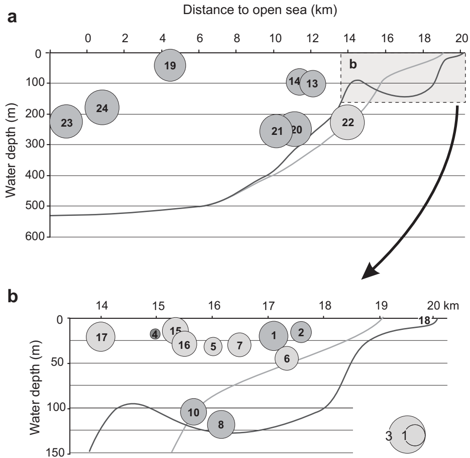
Fig. 9. Shannon diversity index H = -\sum(n_i/n) \ln(n_i/n) calculated for all samples. Note bubble scale expressed by circle surface and gray lines showing bathymetrical profiles along the fjord main axes, dark gray for the main channel and Ezcurra Inlet, bright gray for Martel Inlet.
