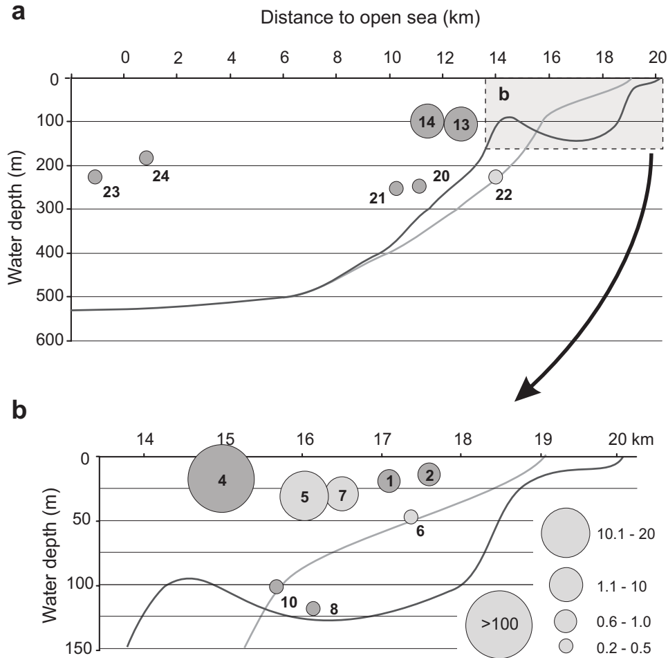
Fig. 8. Total abundances of the monothalamous assemblages expressed in number of specimens per \text{cm}^2 versus water depth and distance to open sea. Data only for the Van Veen and tube-sampler samples. Note non-linear bubble scale used and gray lines showing bathymetrical profiles along the fjord main axes, dark gray for the main channel and Ezcurra Inlet, bright gray for Martel Inlet.
