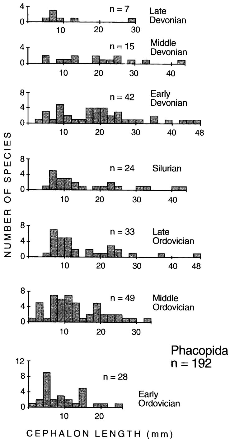
Fig. 6. Frequency distribution of cephalon length of Phacopida species in various intervals of their evolutionary history. Data (including stratigraphic range of the clade) from Harrington et al. (1959).
