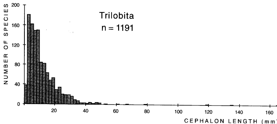
Fig. 8. Distribution of body size in species of Trilobita. Length of the cephalon is used as the size-index. The peak on the side of small sizes results from much higher speciation rate of the smaller species. Data measured from Harrington et al. (1959).
