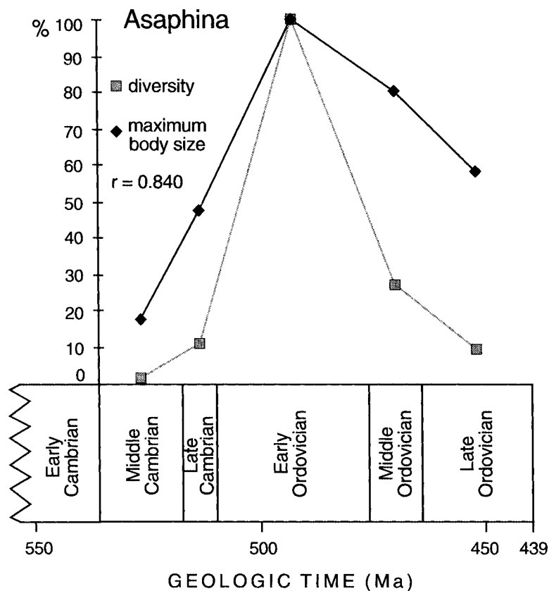
Fig. 5. Changes of the maximum body size compared to changes of the diversity in Asaphina, plotted as a percentage of maximum. Note the strong correlation between size and diversity ( r = 0.840 ). Data from Fig. 4. Time scale after Harland et al. (1990).
