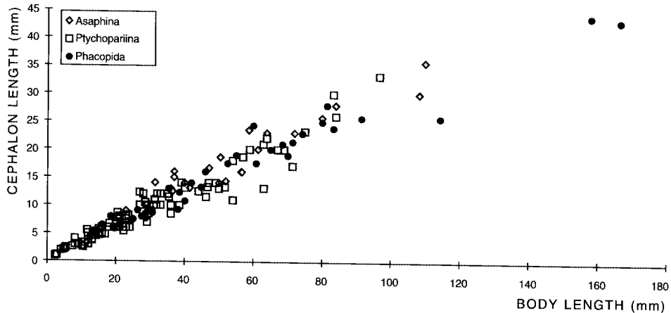
Fig. 1. Body length related to cephalon length in Ptychopariina, Asaphina and Phacopida. Since body length and cephalon length are strongly correlated, length of cephalon can be used as a size-index. Data measured from Harrington et al. (1959).
