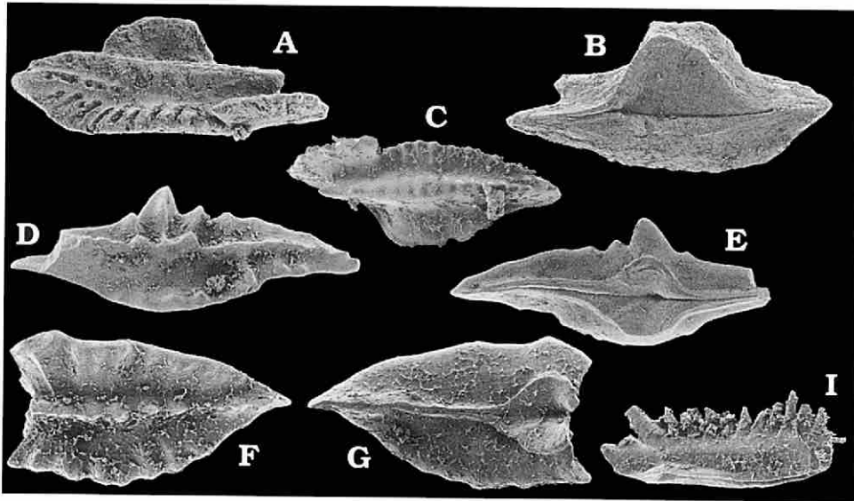
Fig. 5. Conodonts from the Late Tournaisian of the Muhua section (sample Mu-42), Guizhou province, South China. A–B. Mestognathus sp. ZPAL V.XXVI/54 in upper ( A ) and lower ( B ) views. C. Cavusgnathus sp. ZPAL V.XXVI/55 in upper view. D, E. Pseudopolygnathus primus (Branson & Mehl, 1934) in upper ( D ) and lower ( E ) views; ZPAL V.XXVI/56. F, G. Pseudopolygnathus sp. ZPAL V.XXVI/57 in upper ( F ) and lower ( G ) views. I. Prioniodina? sp. ZPAL V.XXVI/58. All are SEM micrographs \times 43 .
